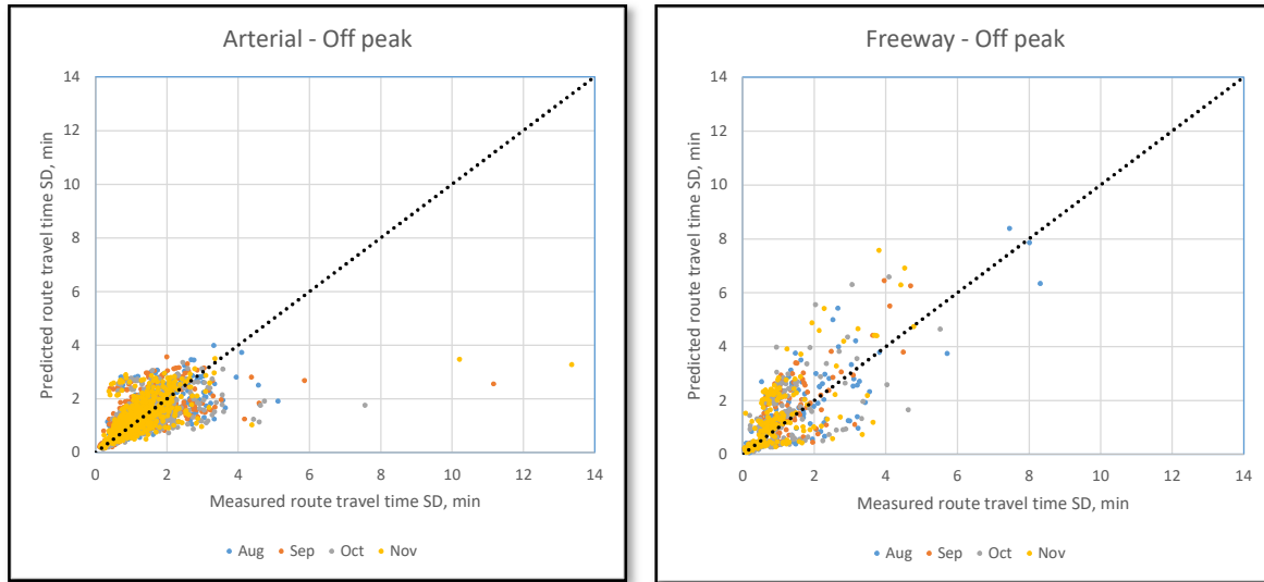
Figure 4-10: Route travel time SD validation across off peak for arterials and freeways
